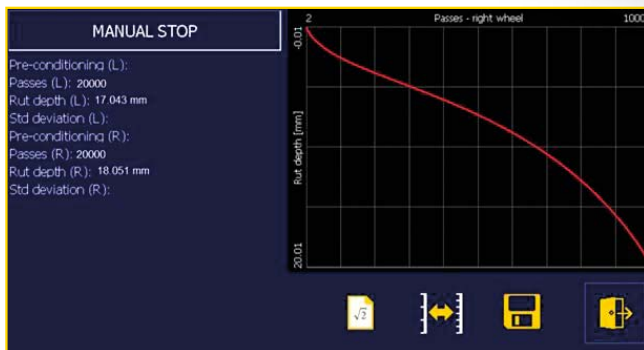
Test execution and all parameters, such as water/air temperature, specimen temperature, rut depth can be monitored in realtime. The software also allows exporting test data to an Excel compatible format
