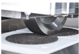
Water and air test at the same time in compliance with EN, BS and AASHTO Standards
